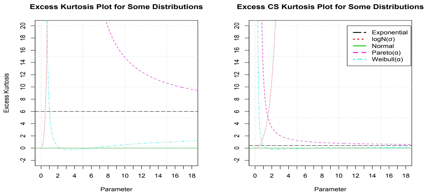
Figure 1: Plots of excess kurtosis vs shape parameter for some distributions
